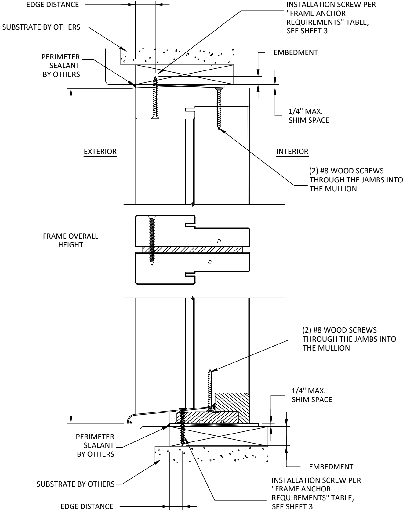
A 3 HORIZONTAL SECTION VERTICAL MULLION
