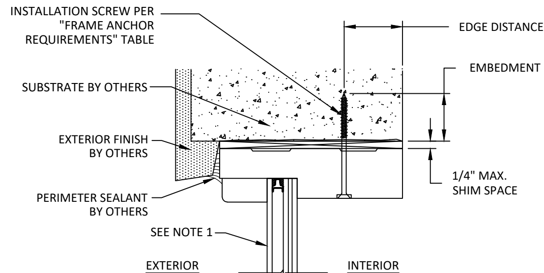
C 2 HEAD SECTION THROUGH FRAME INSTALLATION (SILL & SIDES ARE INSTALLED THE SAME)
