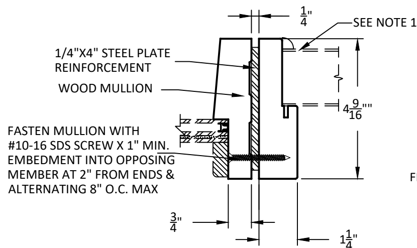
B 2 DIRECT SET SIDELITE VERTICAL MULLION
