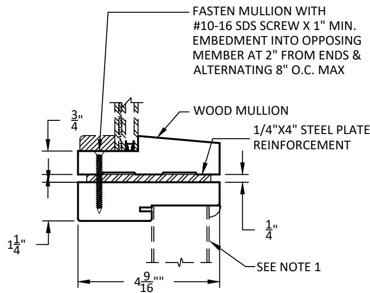
A 2 DIRECT SET TRANSCOM HORIZONTAL MULLION
