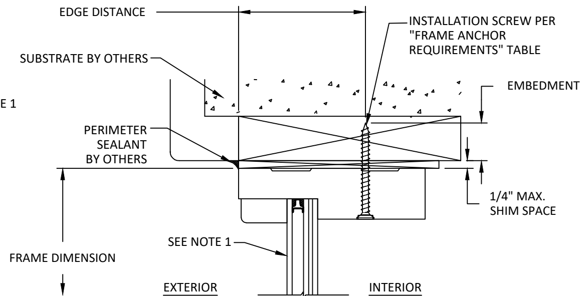
C 2 HEAD SECTION THROUGH FRAME INSTALLATION (SILL & SIDES ARE INSTALLED THE SAME)
