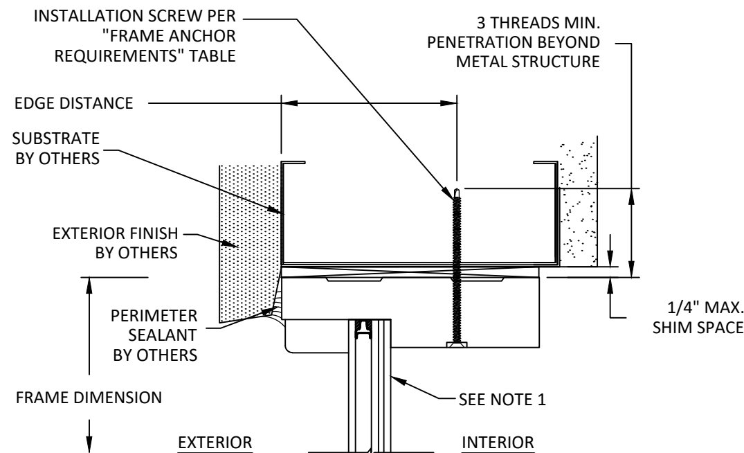
D 2 HEAD SECTION THROUGH FRAME INSTALLATION (SILL & SIDES ARE INSTALLED THE SAME)
